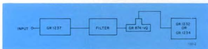
Figure 1. Detector system using the Type 1237.
