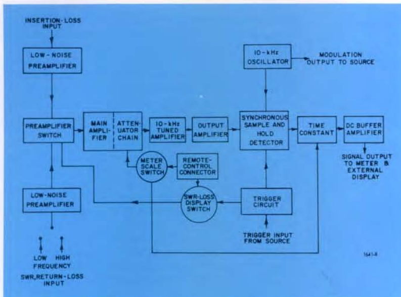
Figure 10. Block diagram of 1641 Indicator.
