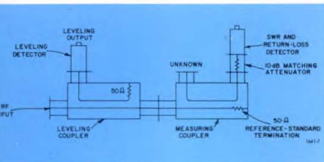
Figure 4b. Schematic diagram of high-frequency unit.
