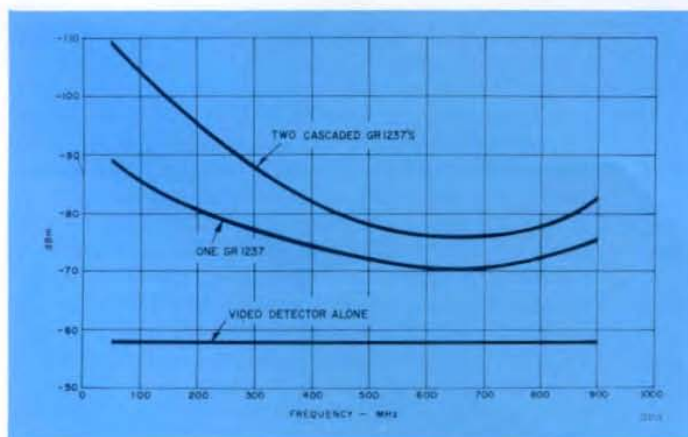
Figure 2. Relative improvement in sensitivity, using the Type 1237.
