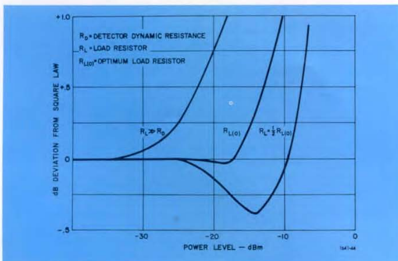
Figure 11. Diode detector — square-law range extension.
