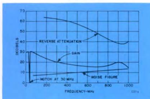
Figure 3. Typical noise figure, gain and reverse attenuation characteristics.
