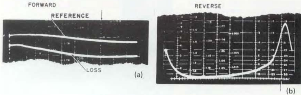
Figure 15. Insertion loss for isolator in the 2.0- to 4.0-GHz range; full scale: 0 dB in 15a and 17 dB in 15b.
