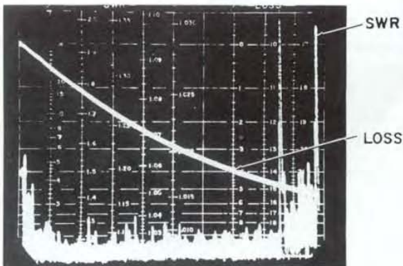
Figure 24. Inertion loss and SWR for 50 feet of RG-214/U cable in the 2.0- to 4.0-GHz range; full scale = 1.10 (SWR) and 10 dB (loss).
