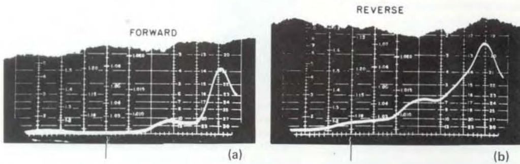
Figure 16. SWR for isolator in the 2.0- to 4.0-GHz range; full scale = 1.35.
