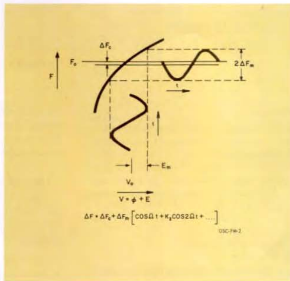
Figure 2. Frequency-modulation characteristic (exaggerated curvature).
